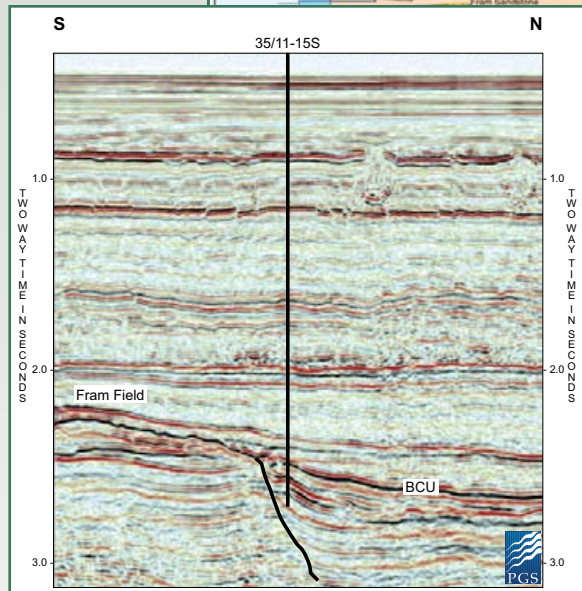
Seismic profile
