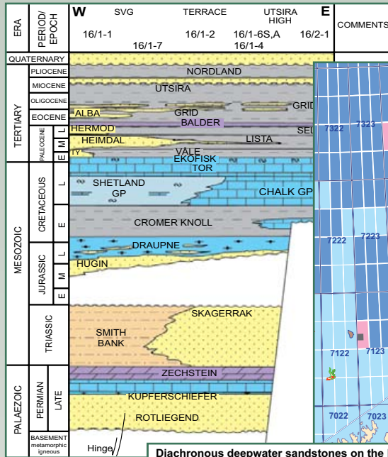
Stratigraphy
